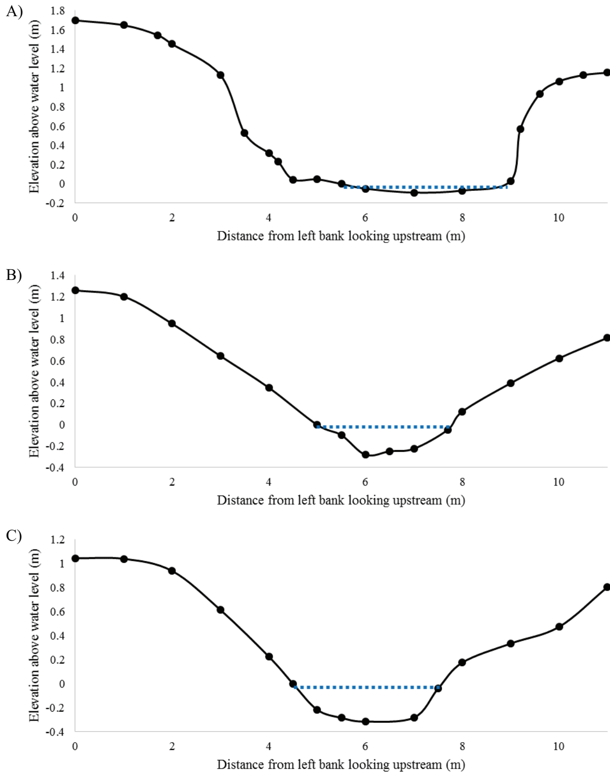
Appendix E-2. Unnamed Drain 2 cross-sectional profiles for the A) lower, B) middle, and C) upper reaches of the drain.
