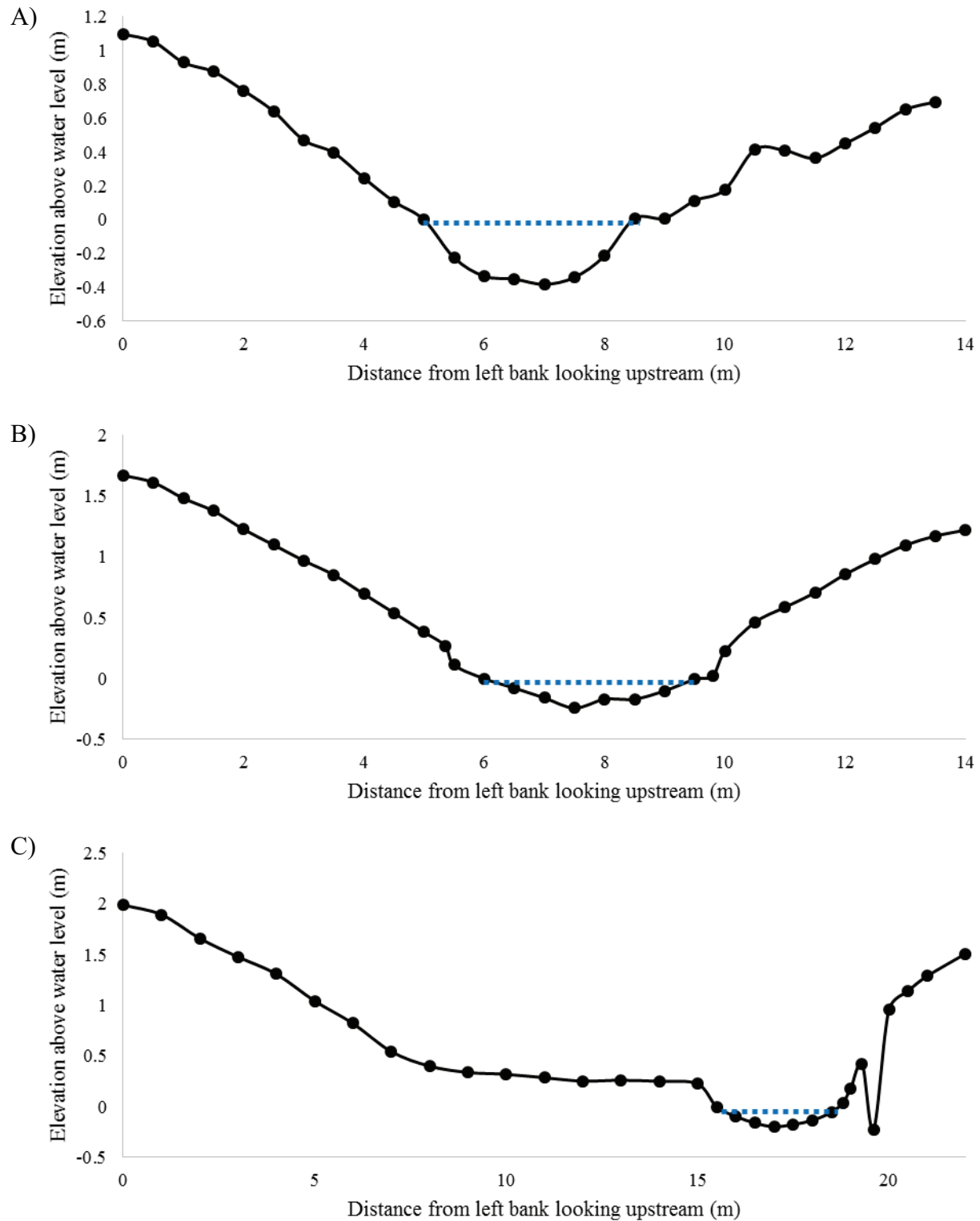
Appendix E-1. Unnamed Drain 1 cross-sectional profiles for the A) lower, B) middle, and C) upper reaches of the drain.
